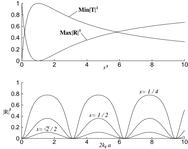
Figure 7: Transmission and reflection coefficients for a rectangular shelf
