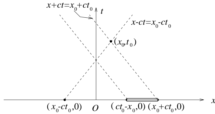
Figure 6: Reflection from a fixed end
