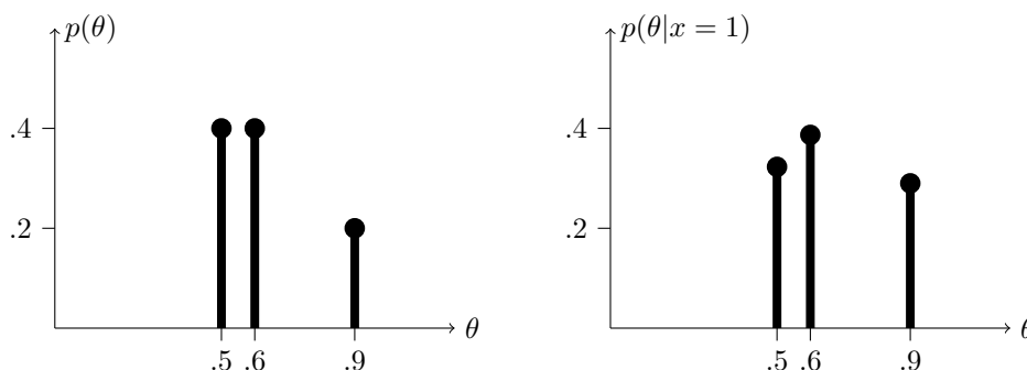
Prior pmf p(\theta) and posterior pmf p(\theta|x = 1) for Example 1
