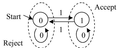
Figure 9: This FA determines if there are an even or odd number of 1's in our data stream.
