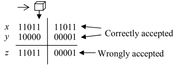
Figure 11: By using the Pigeonhole principle, we can show that we can split two strings at their reflection points such that a finite automaton will be in at the same state for both sub strings. We can then cross the two strings to form a new string that “tricks” the machine into thinking that it has correctly accepted a string as a palindrome.
