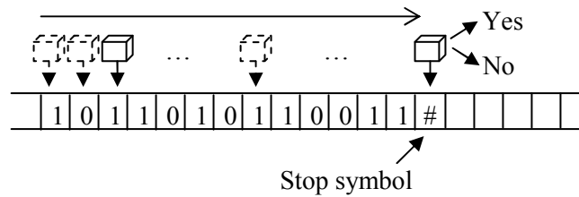
Figure 6: At any given time, the machine has some unique state. The machine reads the tape in one motion (in this case left to right) and the state changes depending on the value of the current square. When it reaches the stop state (signaled by the # sign, the machine returns a yes or no answer - an accept or reject state respectively.)
