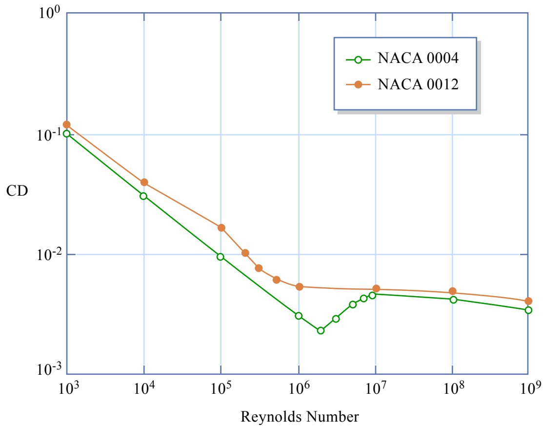
CD vs RE for NACA 0004 and NACA 0012 Airfoils
